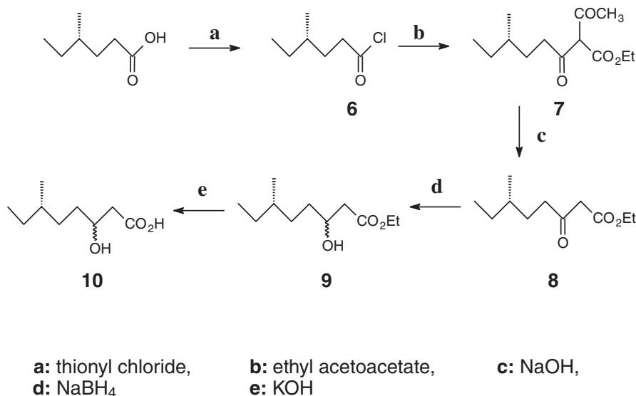
Fig. 2. Synthesis of (3 RS , 6 S )-3-hydroxy-6-methyloctanoic acid.
