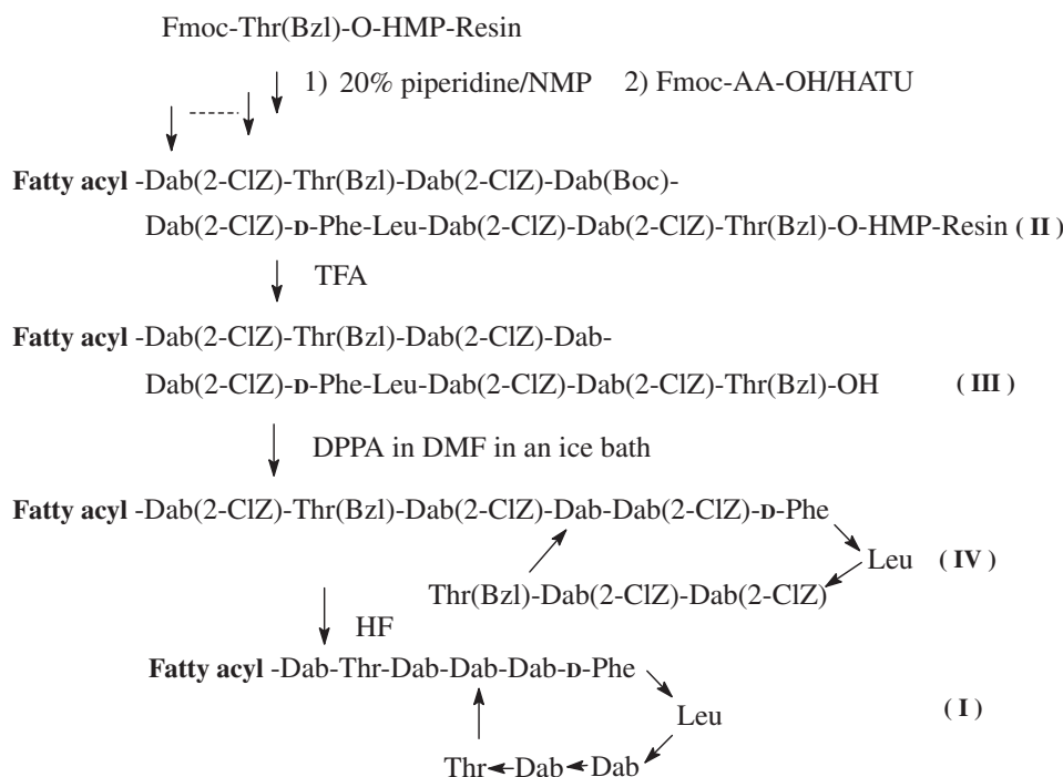
Fig. 3. Synthesis of polymyxin B peptides.
